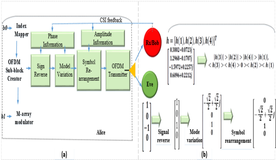
Figure 7. The secure OFDM-IM describes: (a) model; and (b) security sub-block generation, when k = 4, k = 2, M = 2 , and adopt PSK signaling selection strategy and mode.
